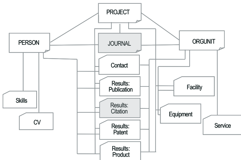
Figure 2. Position of LPJs in CERIF as applied in CRIS-TraM
