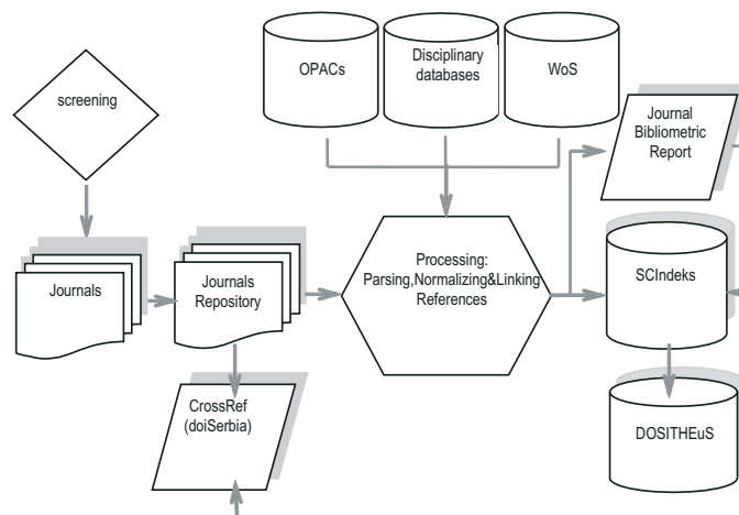
Figure 3. Journals data processing and utilizing in DOSITHEuS
